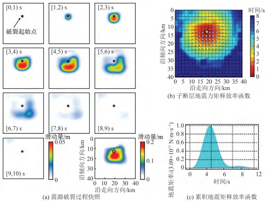
图 5 断层面动态破裂图 Fig. 5 Dynamic Rupture Process on the Fault
